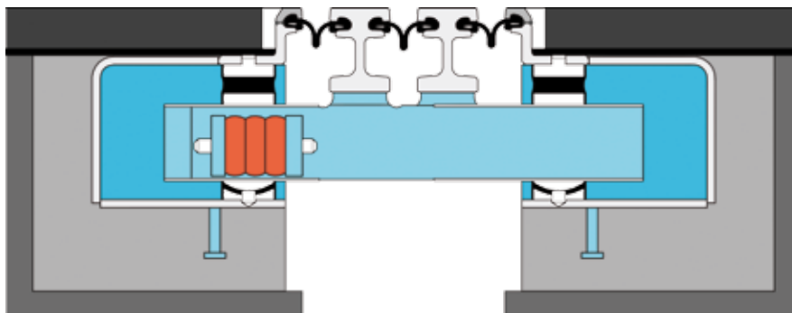
Girder Grid Joints (noise reduction included / not included) Technical Approval according to TL/TP FÜ
